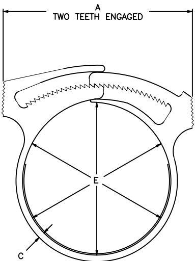
MAXIMUM CAPACITY
