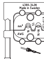
Crimp Profile
