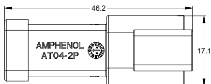
AT04-2P-xxxx
