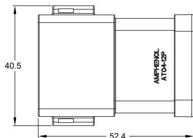
AT04-12Px-xxx
