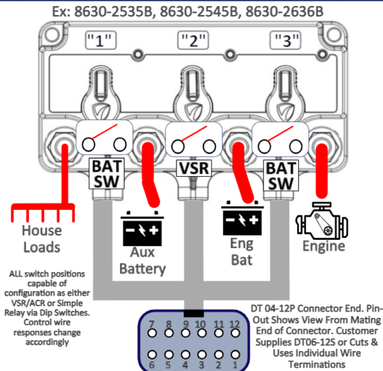
12 Pin Connector Functions (Fig 11)
