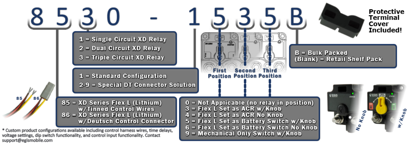
Fig 3 - XD Series Part Number Guide
