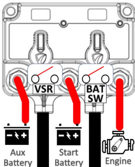
Fig 12 - Dual XD - 85 Series (Flying Wires)
