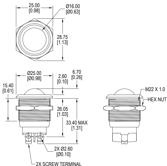
22mm, Round Lens, Screw Terminal
