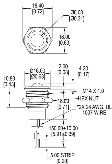
14mm, Round Lens, Wire
