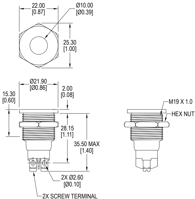
19mm, Flat Lens, Screw Terminal
