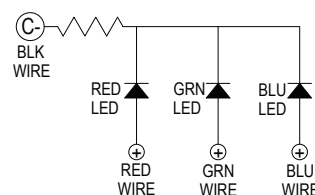
RGBC, with resistor common cathode
