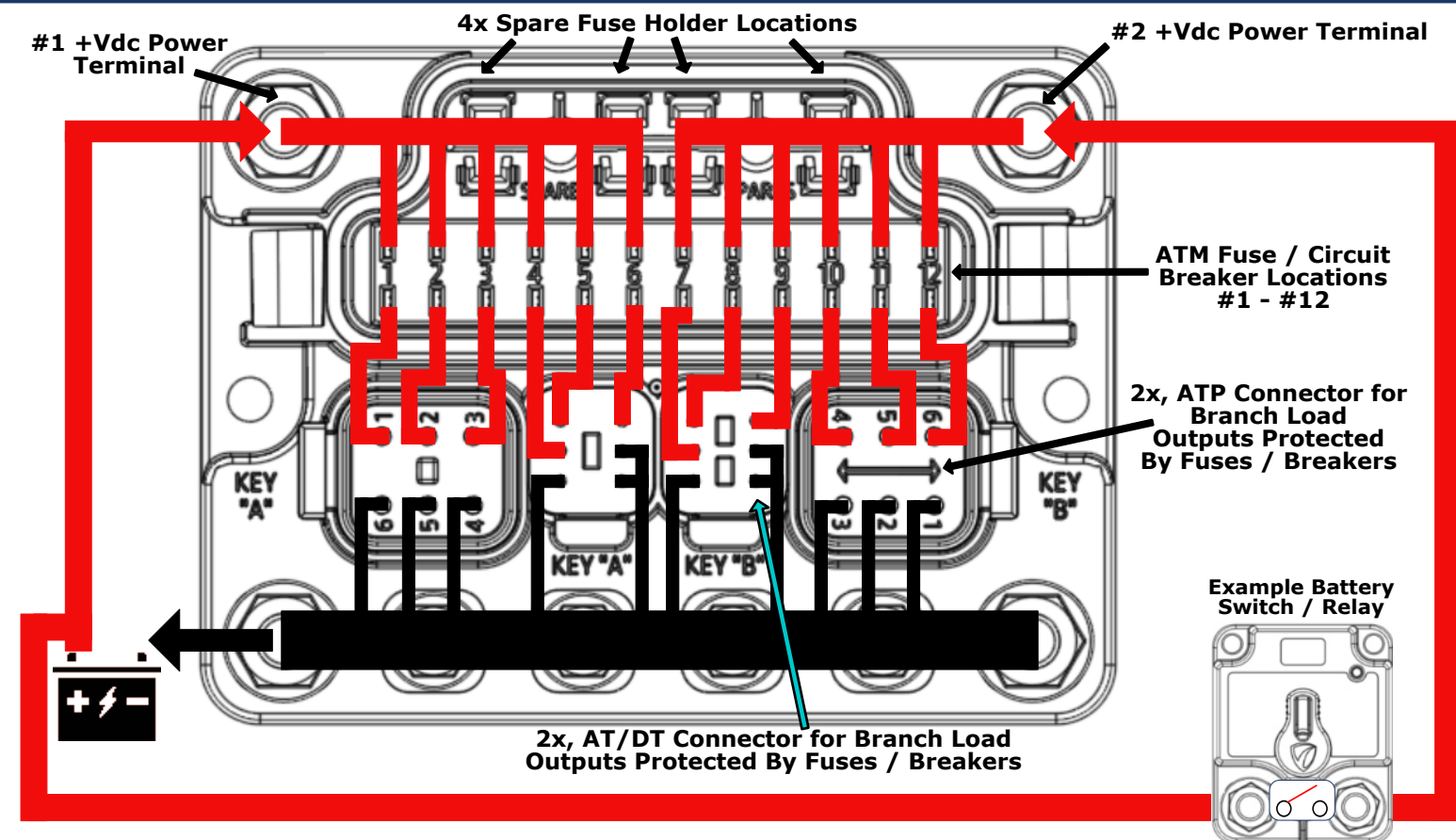
Fig 2 - Internal and Typ External Connections - PN 3466B - Sealed Split Input ATM Block 6 + 6 Circuits
