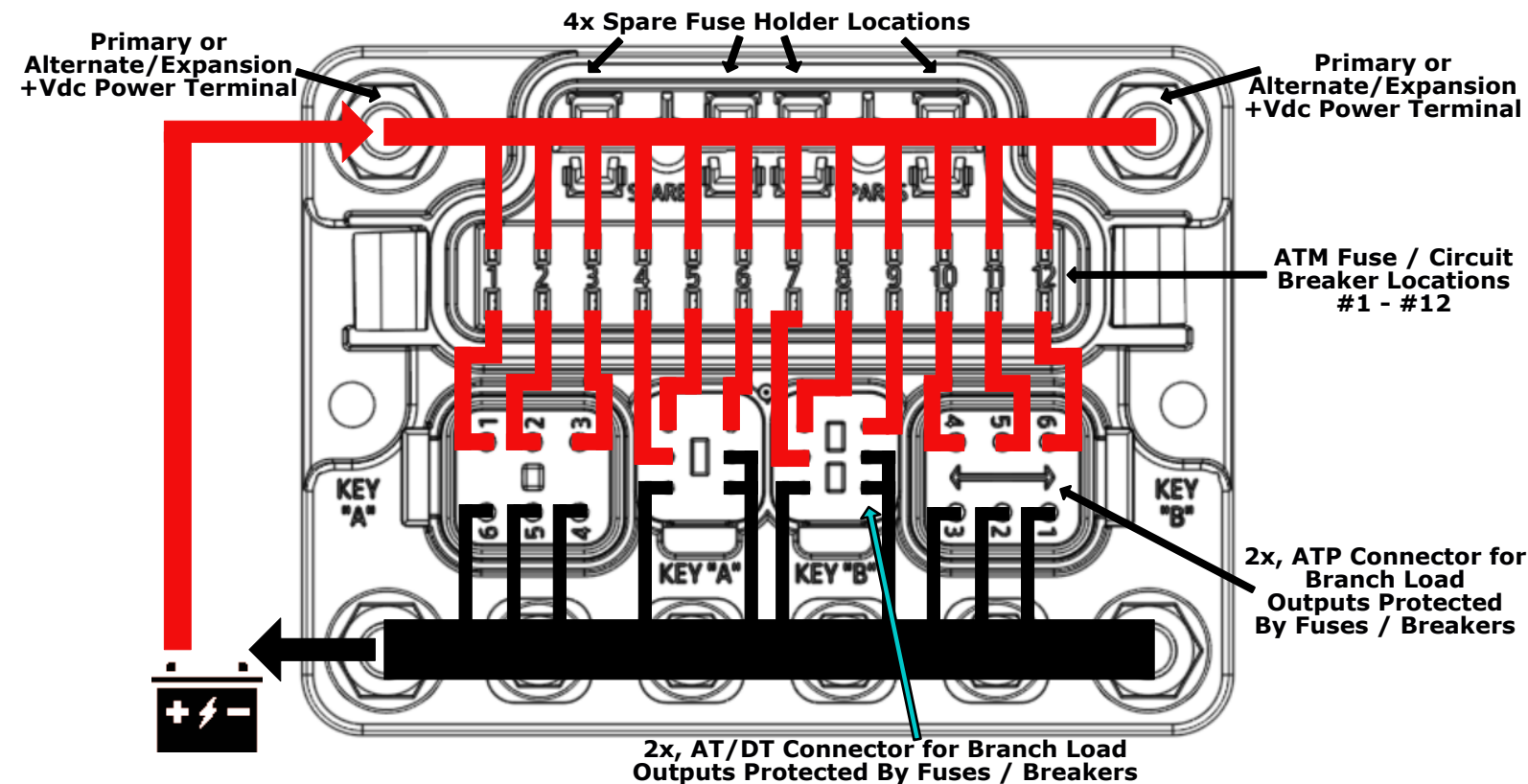
Fig 1 - Internal and Typical External Connections - Sealed ATM Block - Single Input w/Expansion Stud
