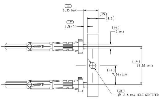
CARRIER STRIP VIEW SCALE 4:1
