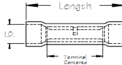
Extruded Vinyl Insulated Seamless Butt Connector
