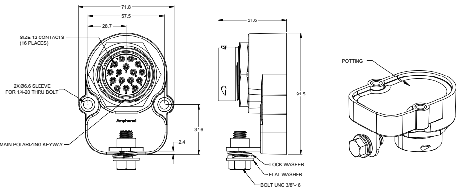
DuraMate™ AHDP with HYPERBUSSTM - Bussed Receptacles For intermateable DuraMate™ AHDP Series plugs (AHP06-), refer to our website
