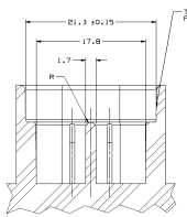
SECTION B - B MATING PART
